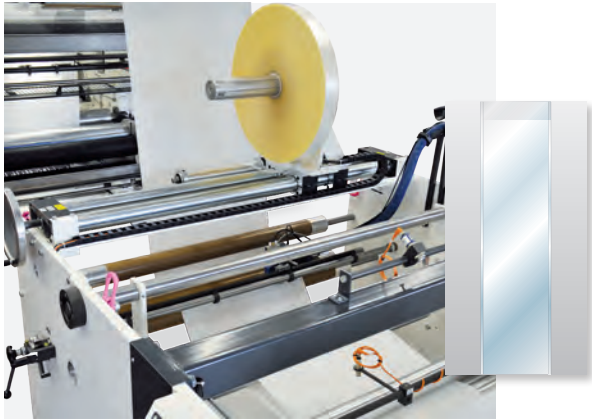
Inline printer LINAFLX NL
